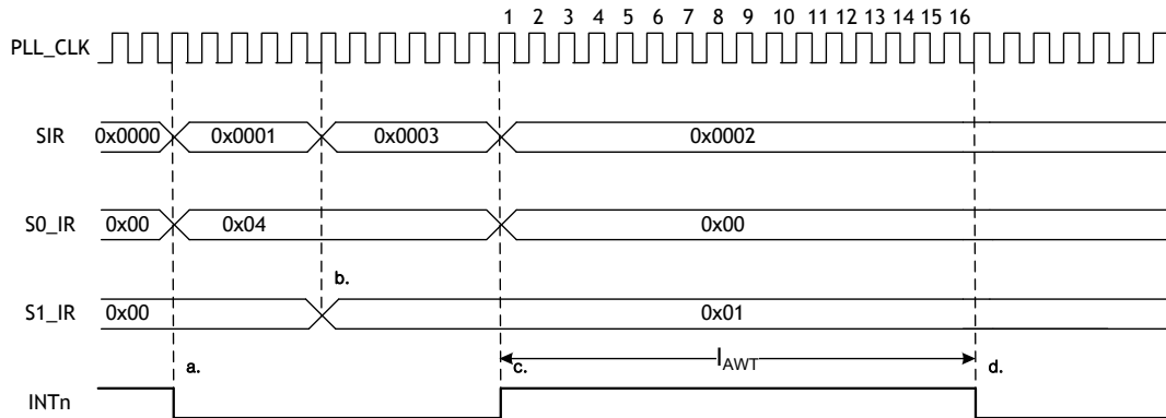
Figure 21. INTLEVEL Timing
