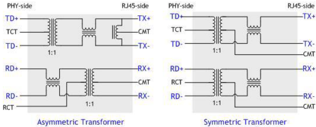
Figure 24. Transformer Type
