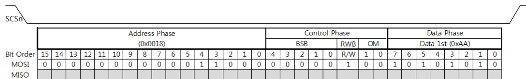
Figure 9. SIMR Register Write in VDM Mode
