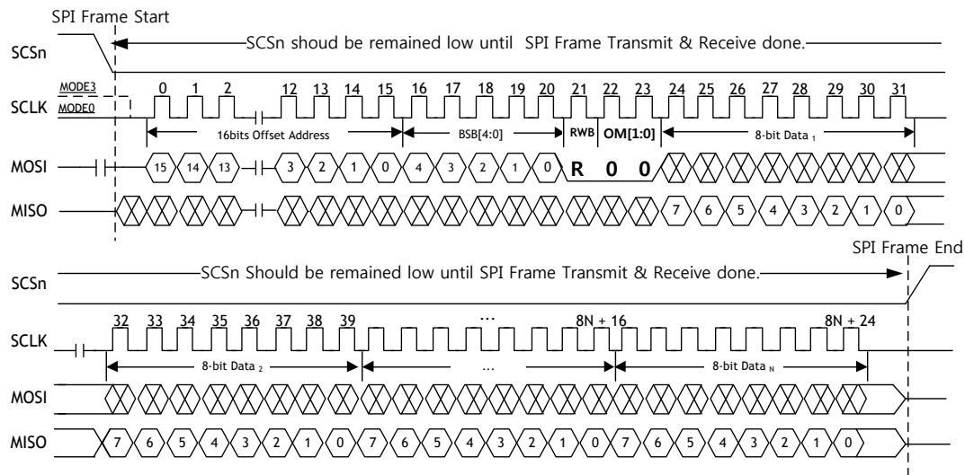
Figure 11. Read SPI Frame in VDM mode
