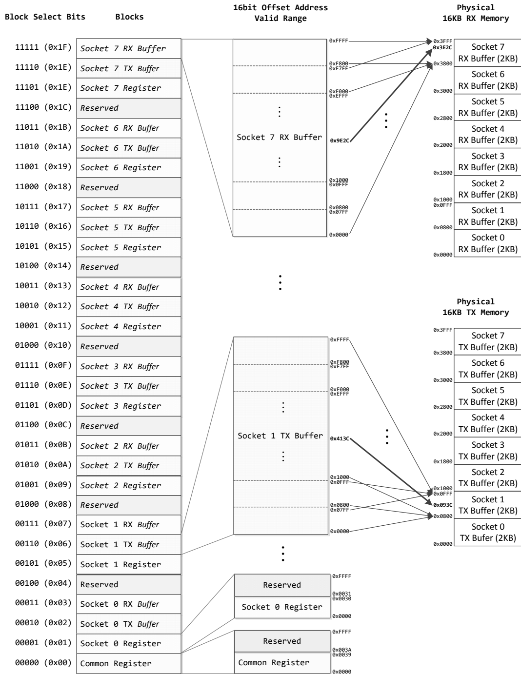
Figure 20. Register & Memory Organization
