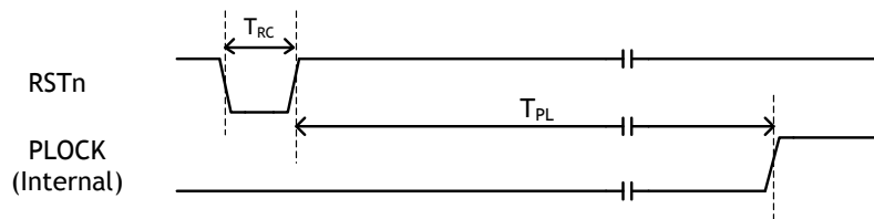
Figure 22. Reset Timing
