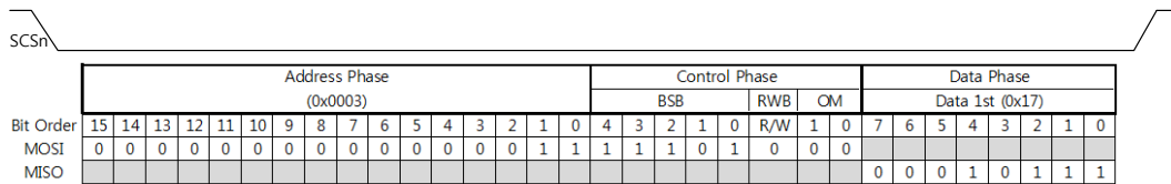
Figure 12. S7_SR Read in VDM Mode
