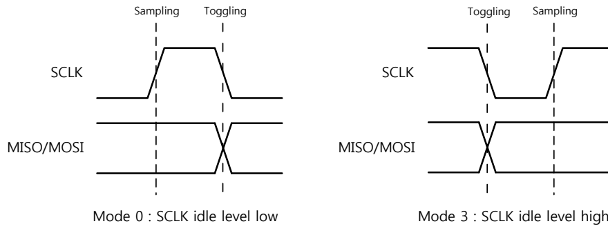
Figure 6. SPI Mode 0 & 3
