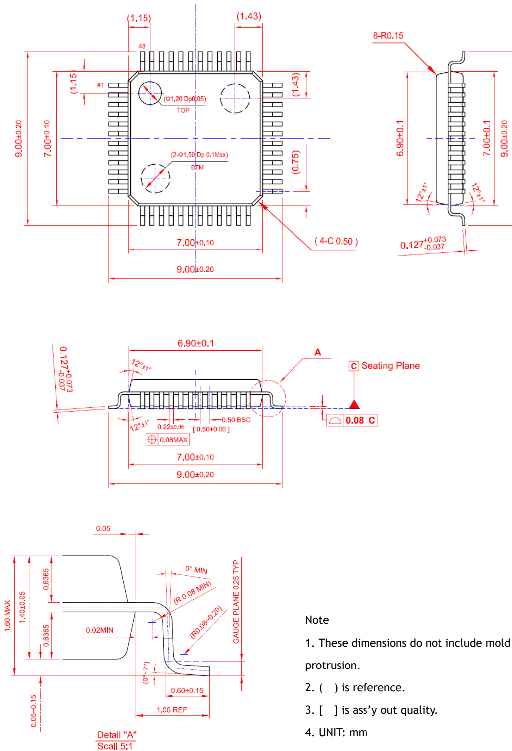
Figure 26. Package Dimensions
