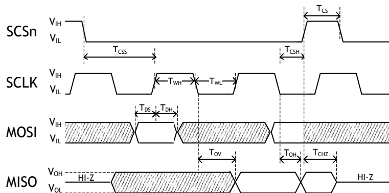
Figure 23. SPI Timing
