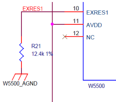
Figure 2. External reference resistor
