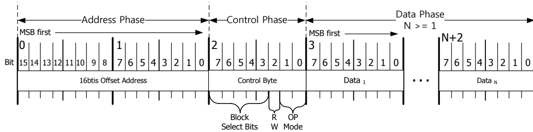
Figure 7. SPI Frame Format
