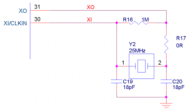
Figure 3. Crystal reference schematic
