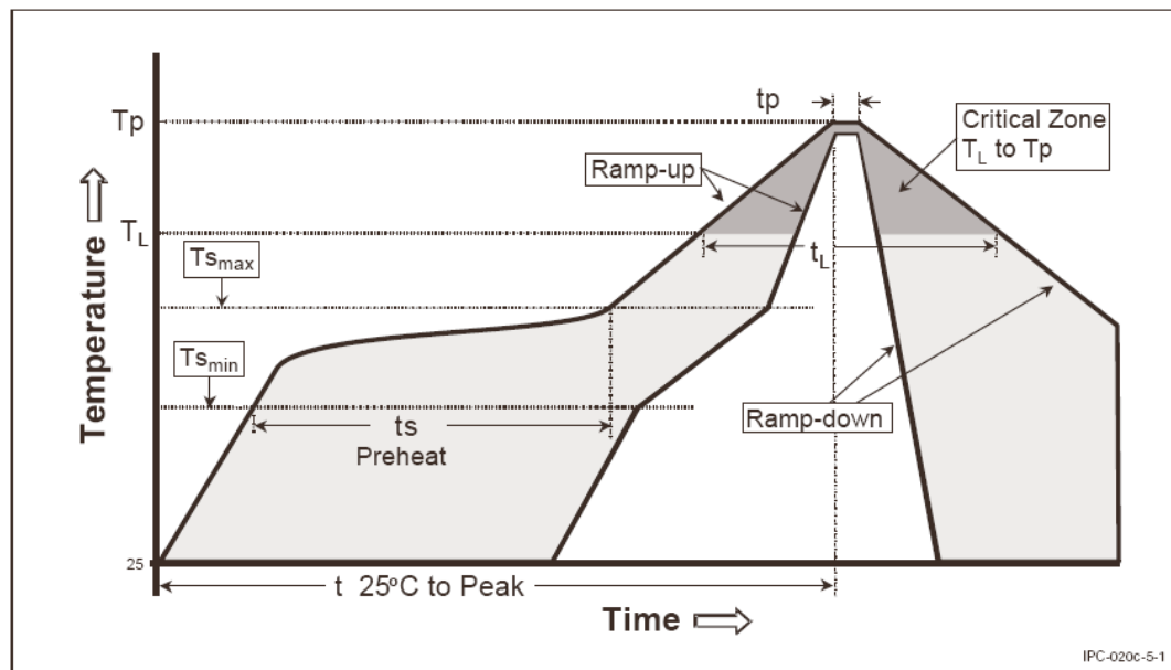
Figure 25. IR Reflow Temperature
