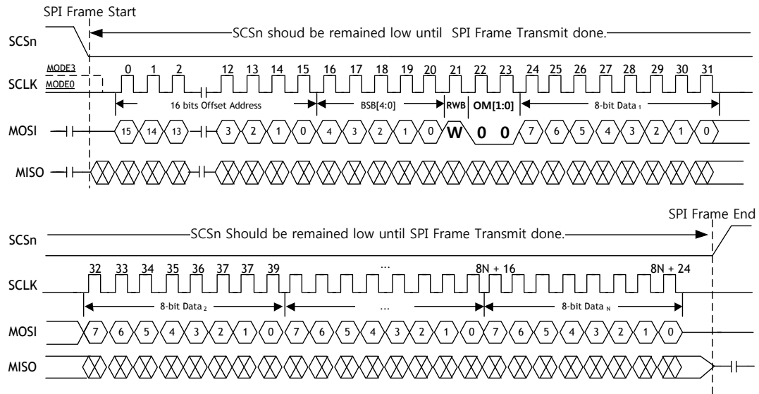
Figure 8. Write SPI Frame in VDM mode
